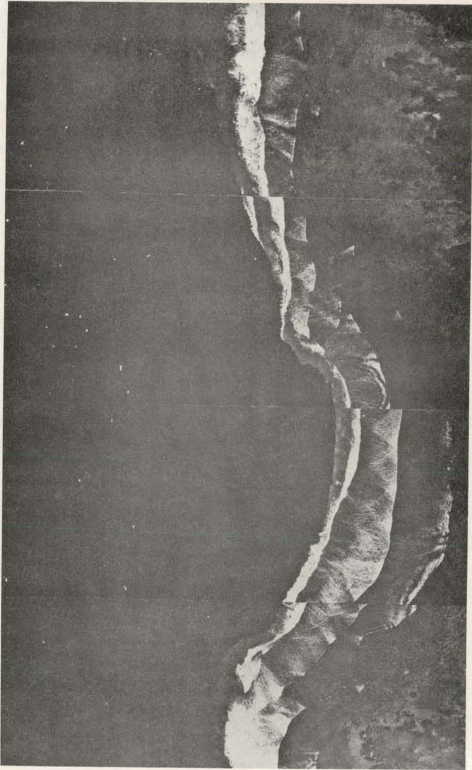
Fig. 47. Break in reef opposite the Mike crater (see Fig. 45).
